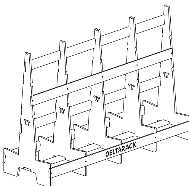
SG60.6.180 / 6 uprights
