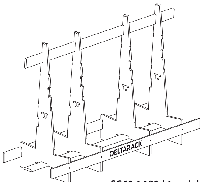
SG60.4.180 / 4 uprights
