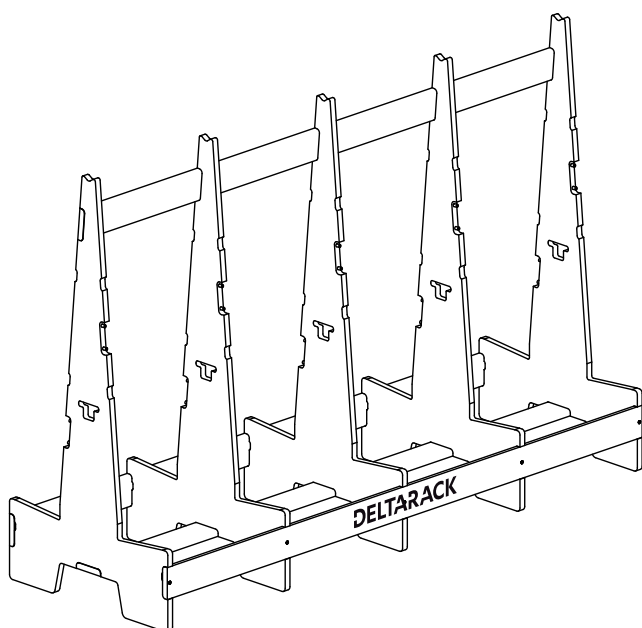
SG60.4.180 / 6 uprights
