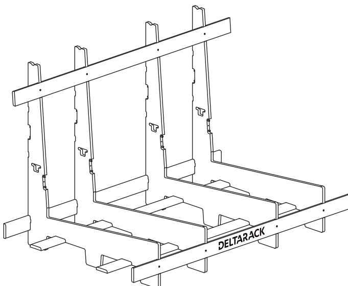
SL110.5.180 / 4 uprights
