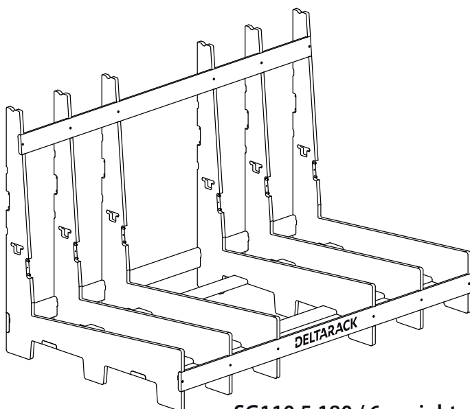
SG110.5.180 / 6 uprights
