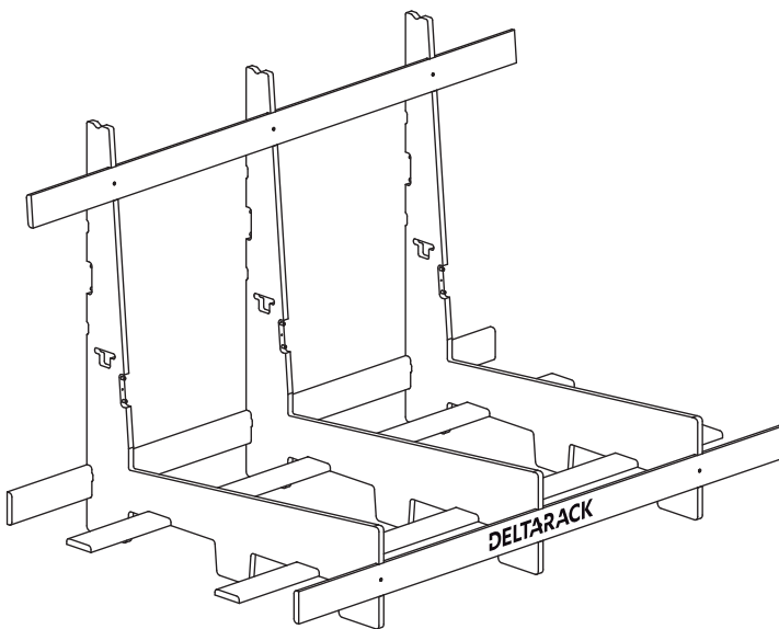
SG110.5.180 / 3 uprights
