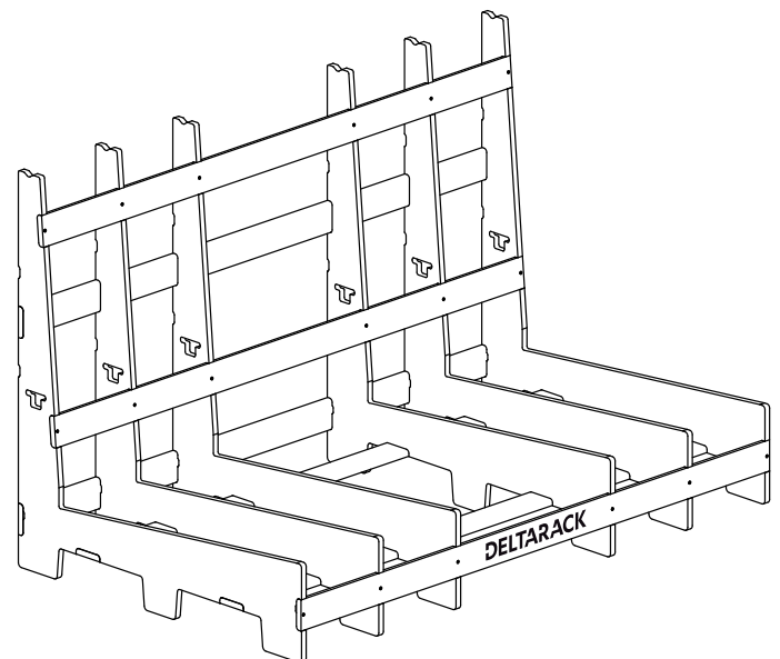
SG110.7.180 / 6 uprights
